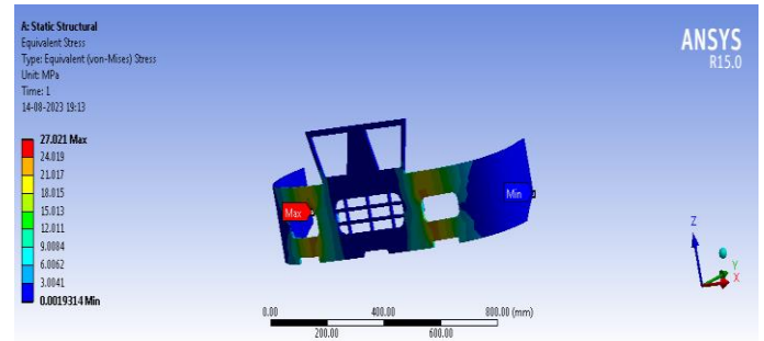
Figure 48 Von-mises stress of Polypropylene material
