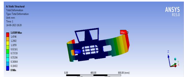
Figure 49 Total deformation of Polypropylene material
